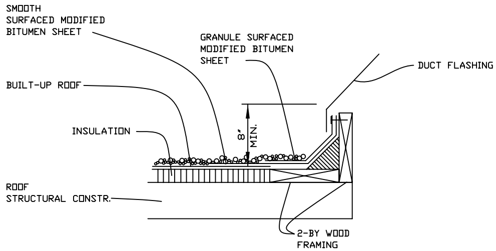
DUCT CURB DETAIL
